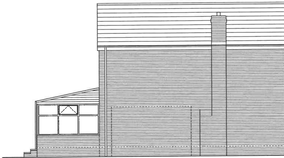
EXISTING NORTH WEST ELEVATION 1:100 @ A4
