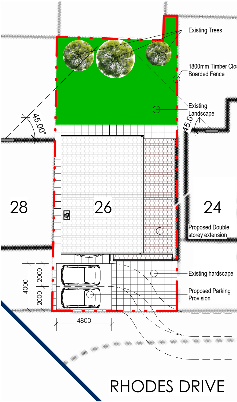
Proposed Site Layout Plan 1 : 200
