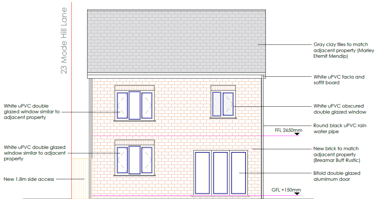
Fig. 6 Rear Elevation
