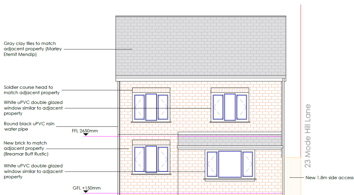
Fig. 5 Proposed front Elevation
