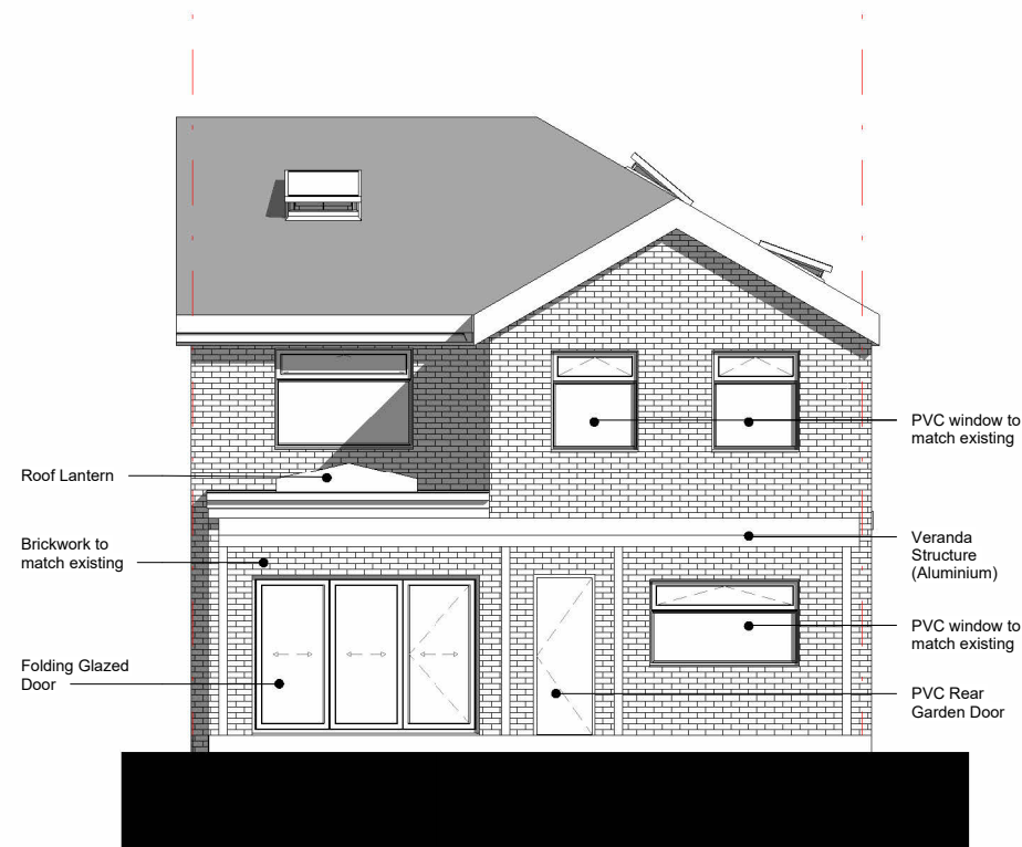
PROPOSED REAR ELEVATION 1:100 @ A3
