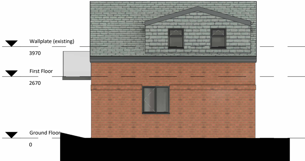
11 Side 2 Proposed 1 : 100
