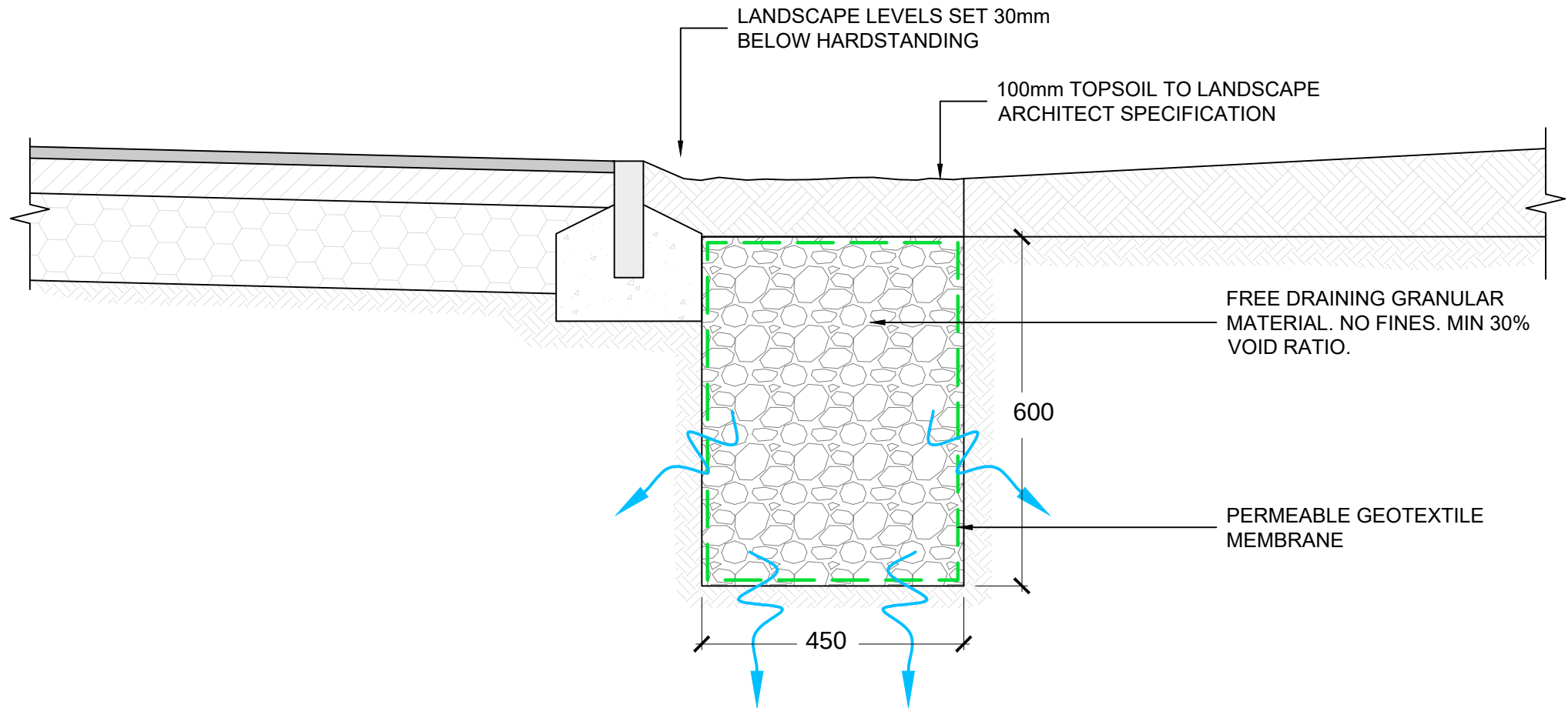
Typical topsoil covered filter drain detail
