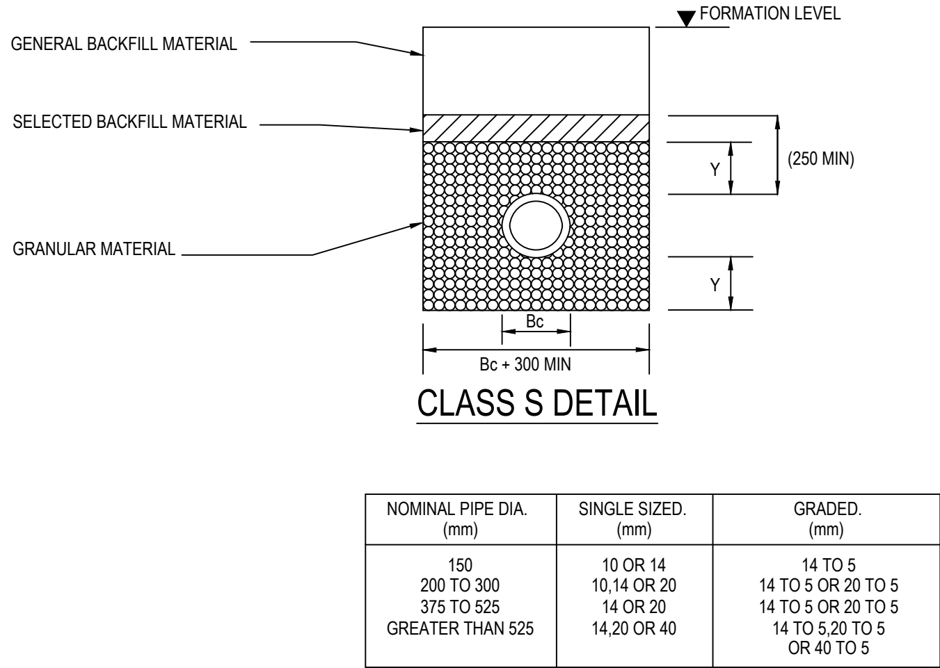
Granular bedding material (ALL AGGREGATES TO TABLE 4 OF BS 882 :1983)
