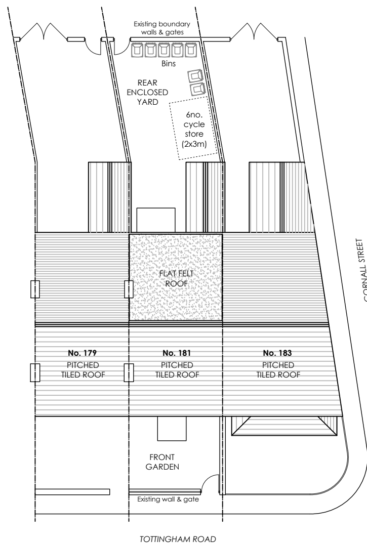
SITE PLAN AS PROPOSED (1:200)
