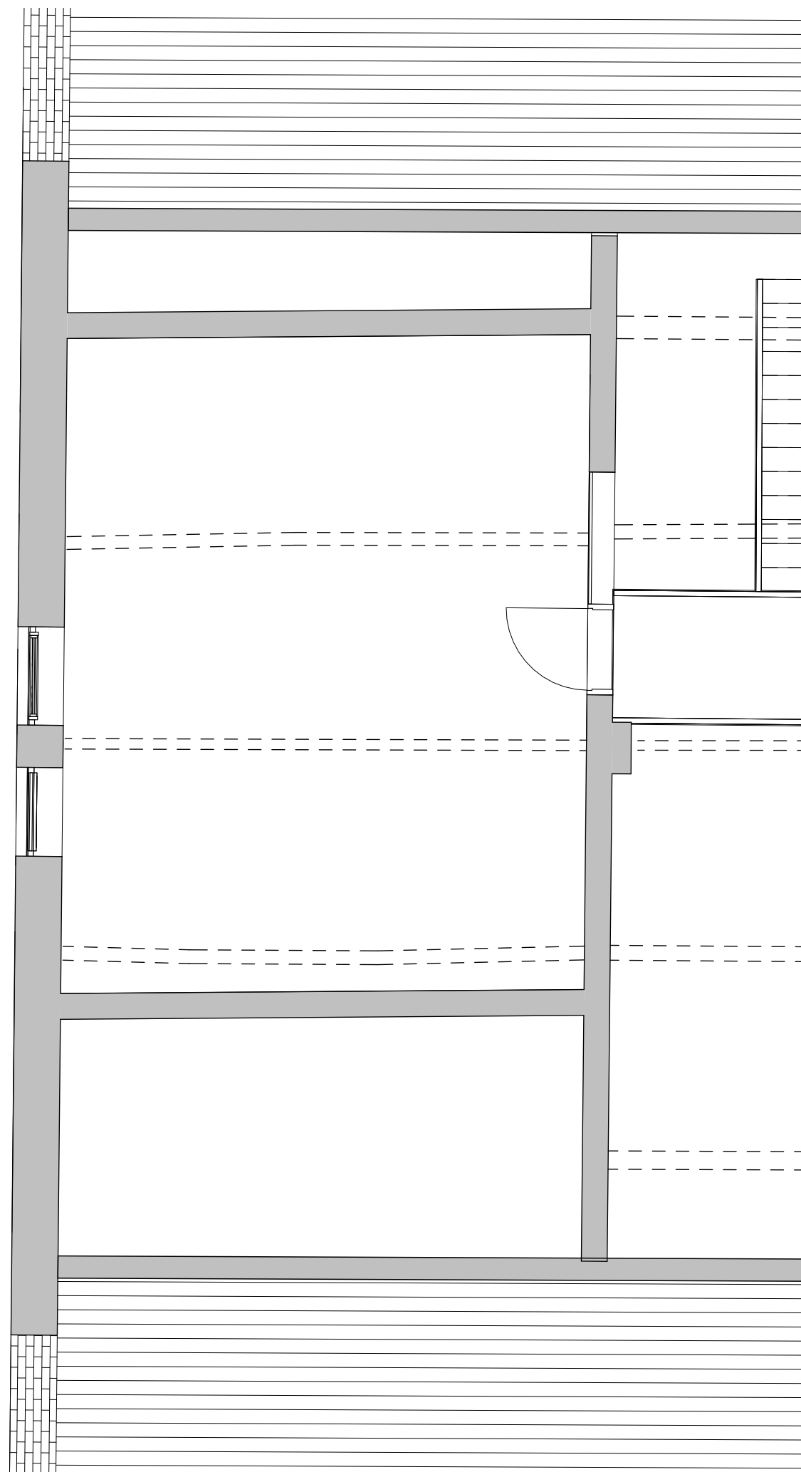
2 Level 2 - Proposed 1 : 50
