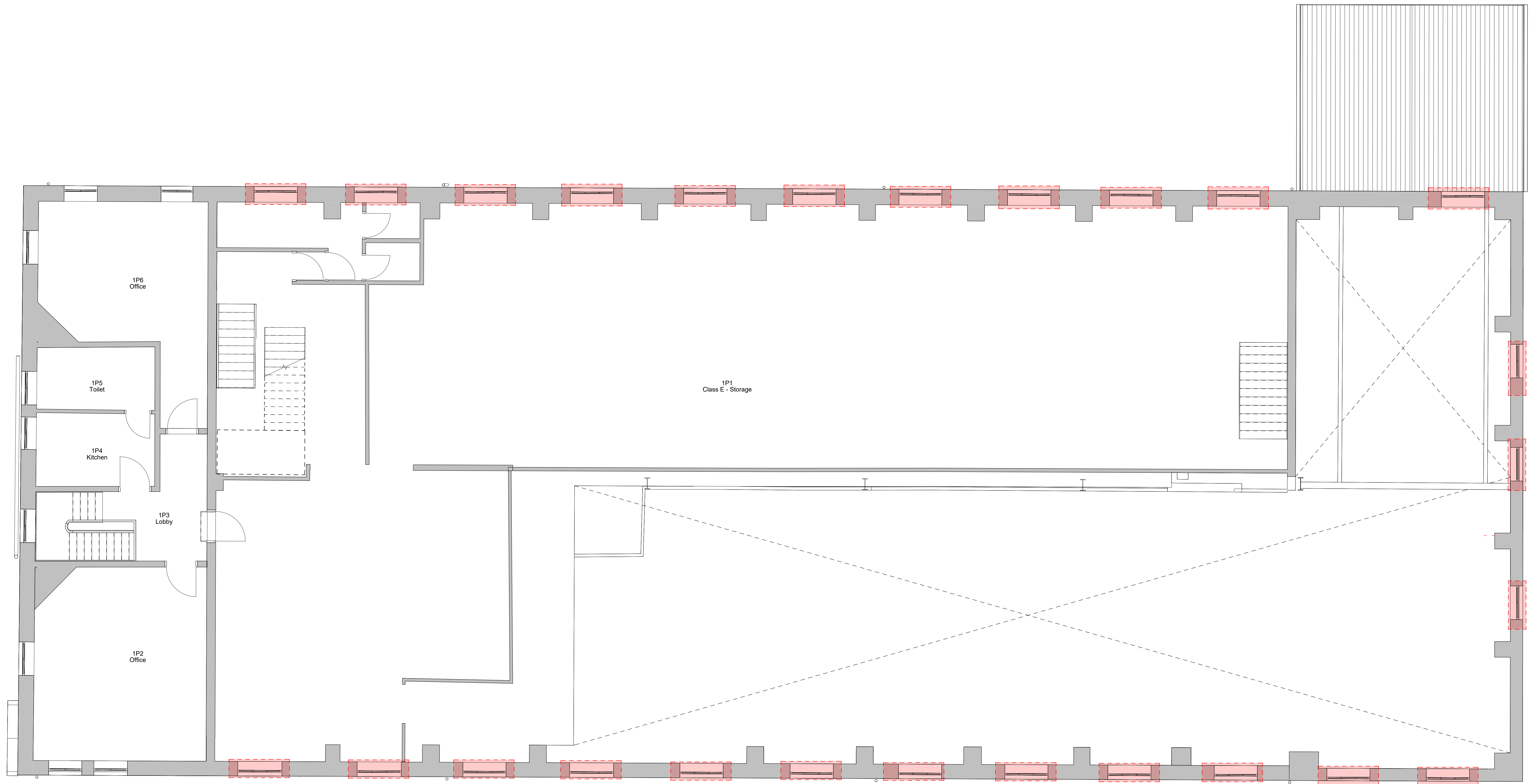
1 Level 1 - New - Proposed 1 : 50
