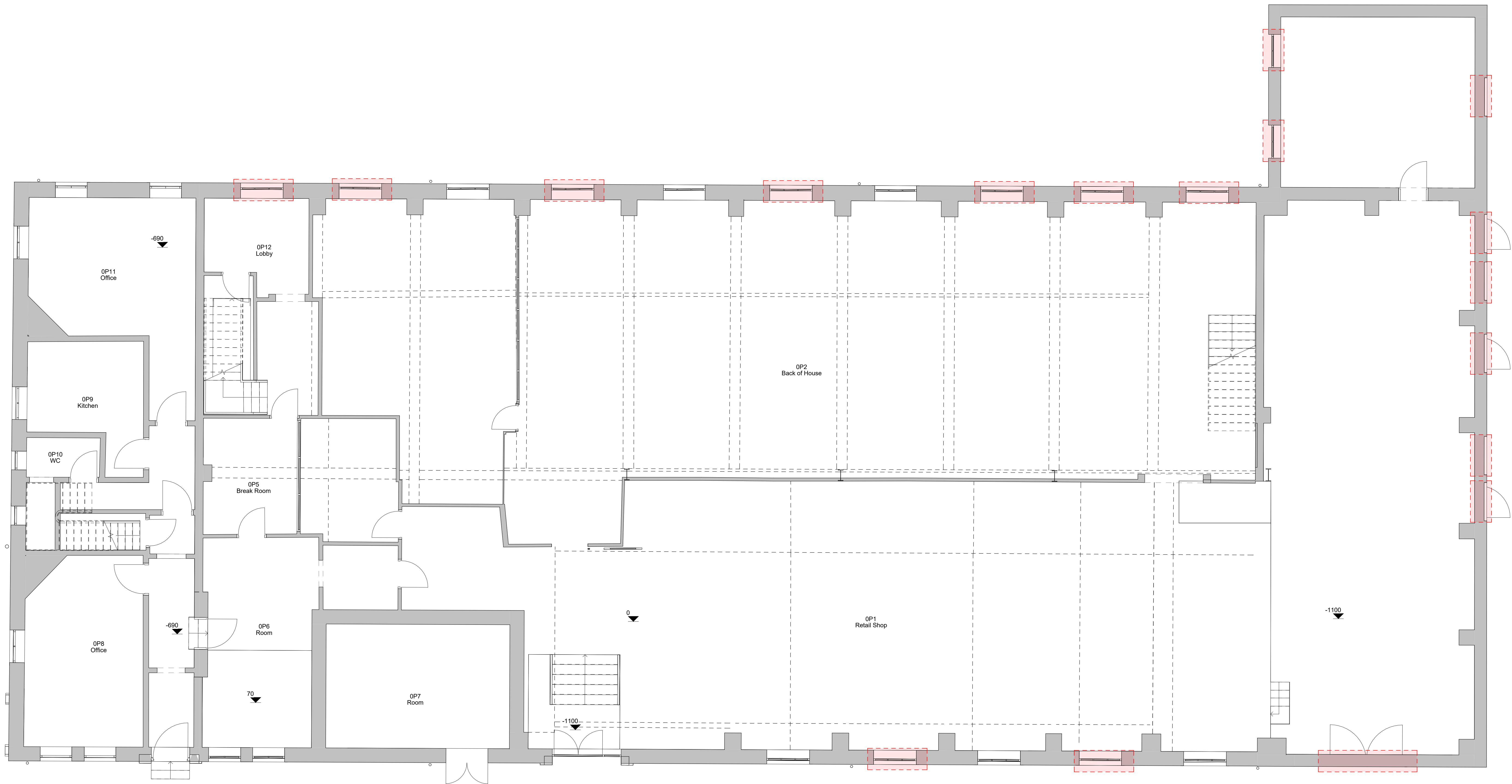
1 Level 0 - Proposed 1:50
