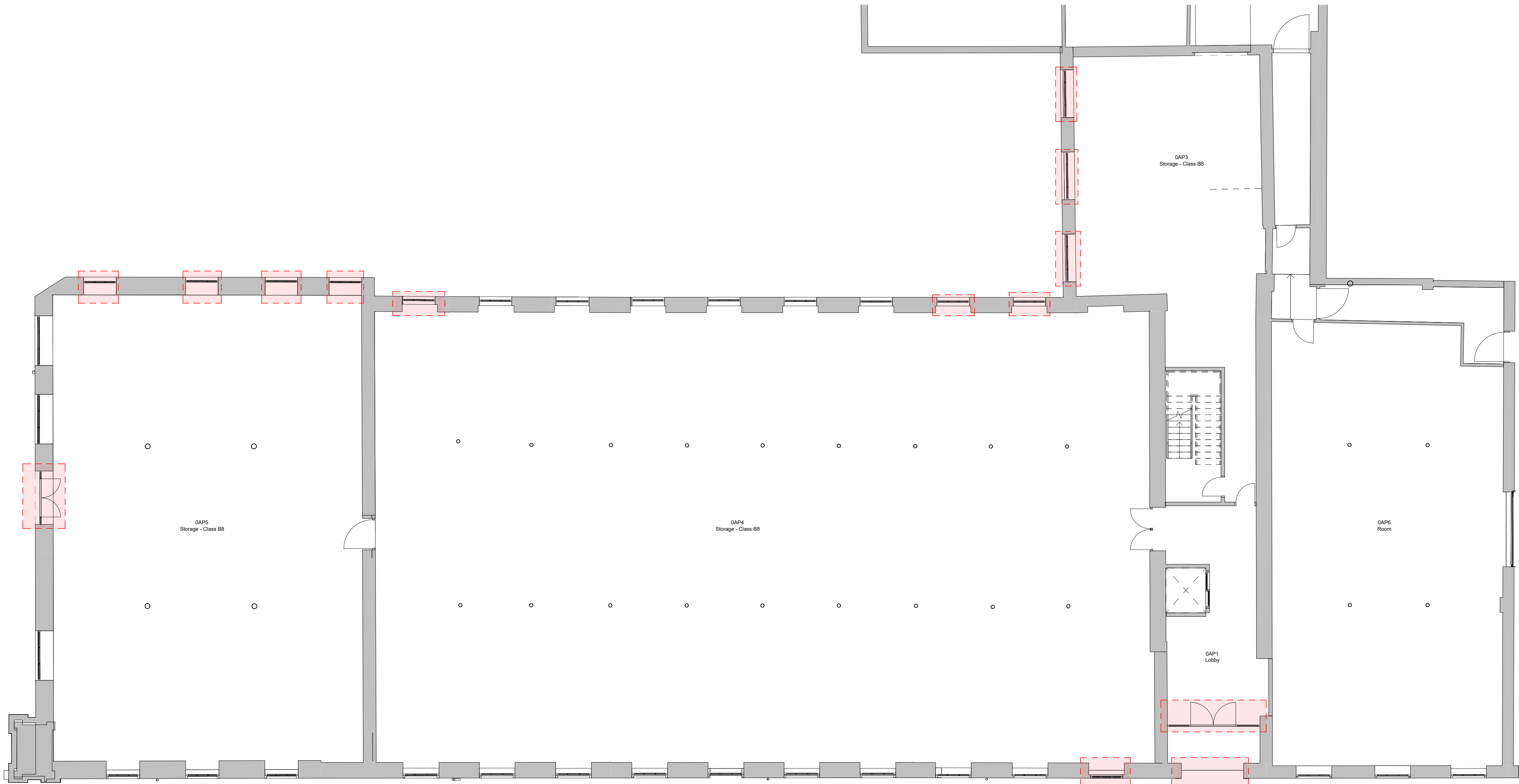
1 Level 0 - Approved Plans 1 : 100
