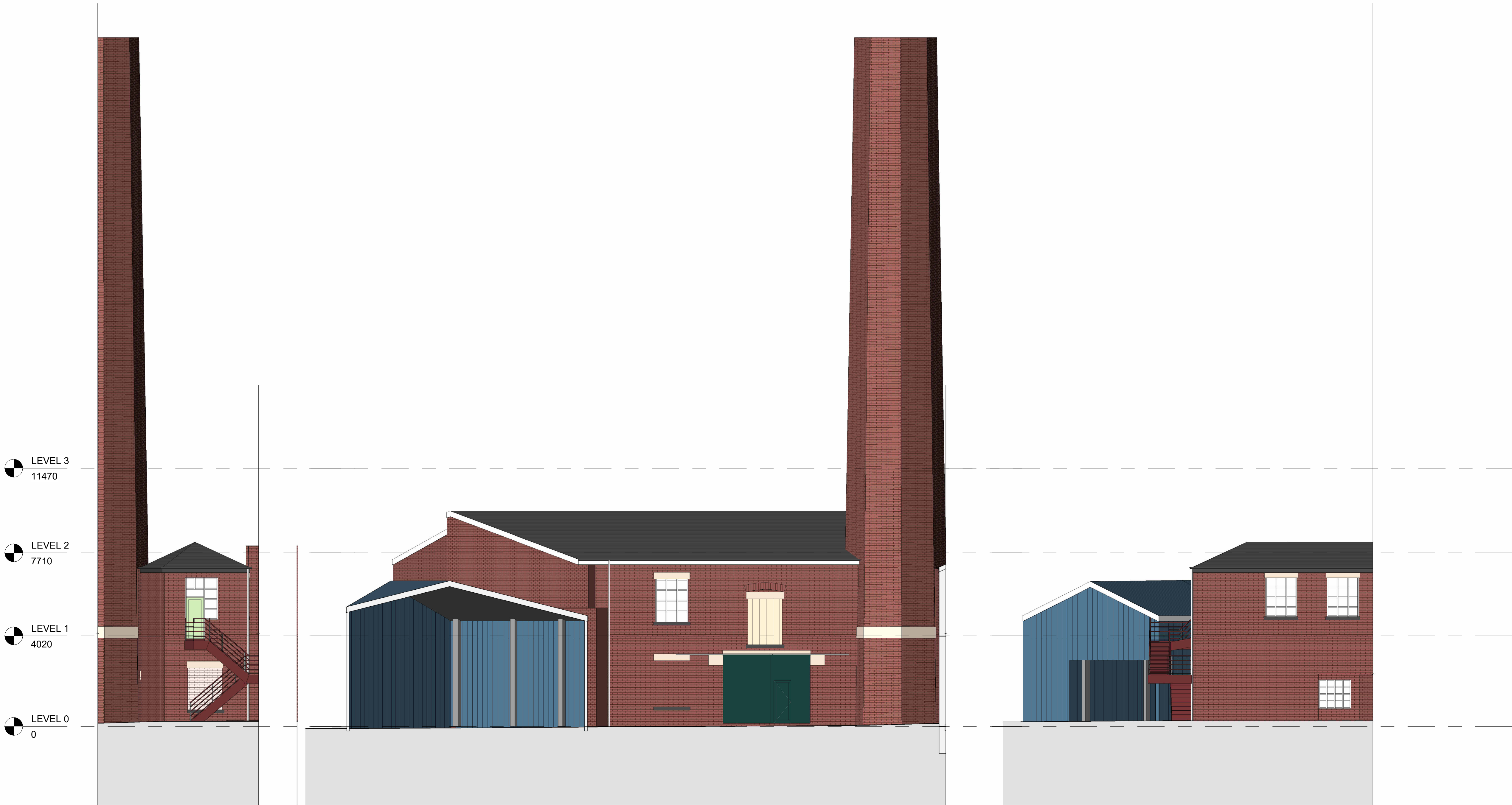
1 Albion Mill Rear - FRONT 1 - Existing 1 : 100
