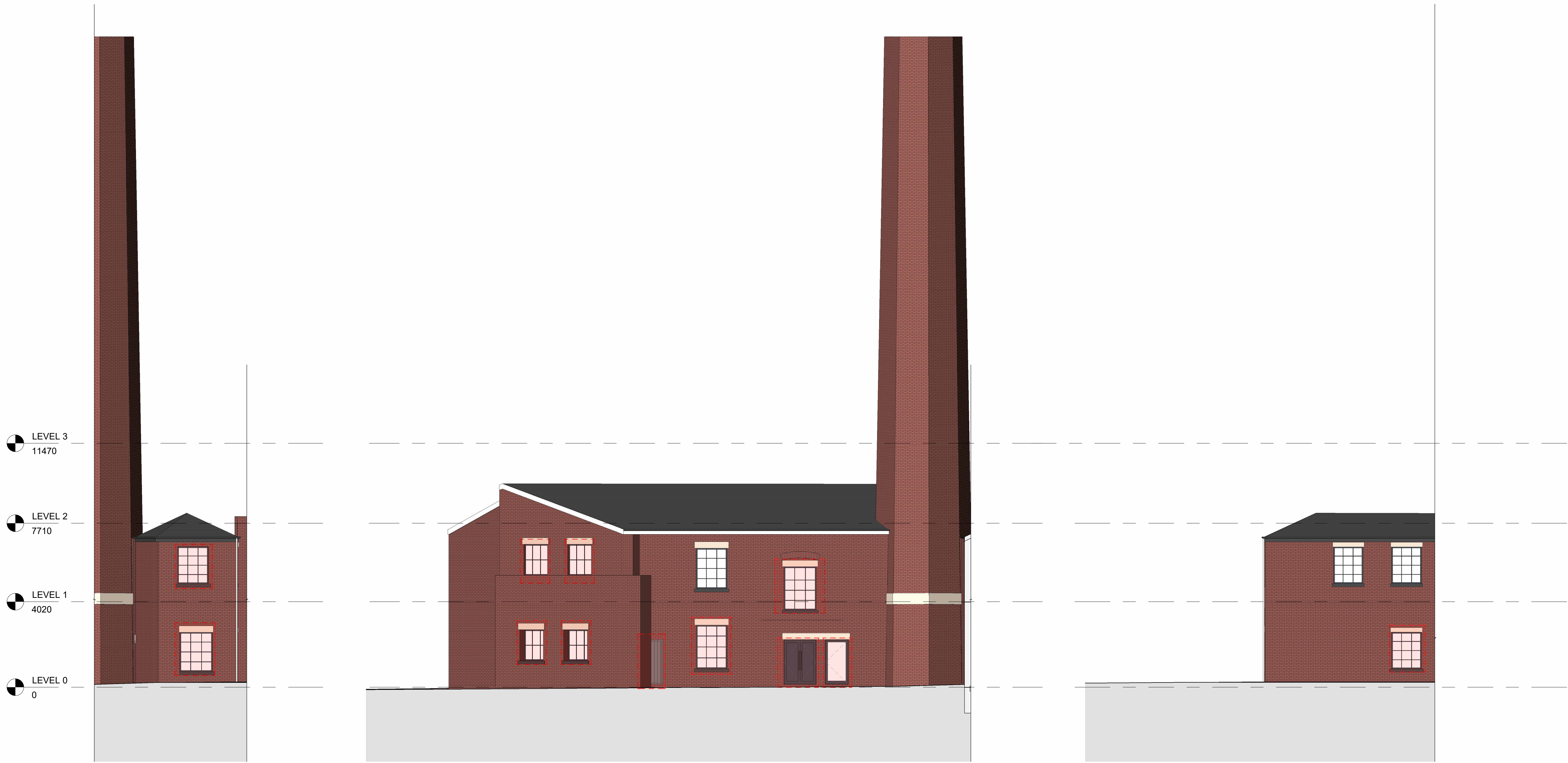
1 Albion Mill Rear - FRONT 1 - Proposed 1 : 100
