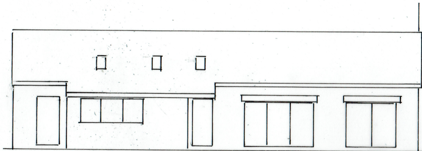
NORTH ELEVATION (UNCHANGED)
