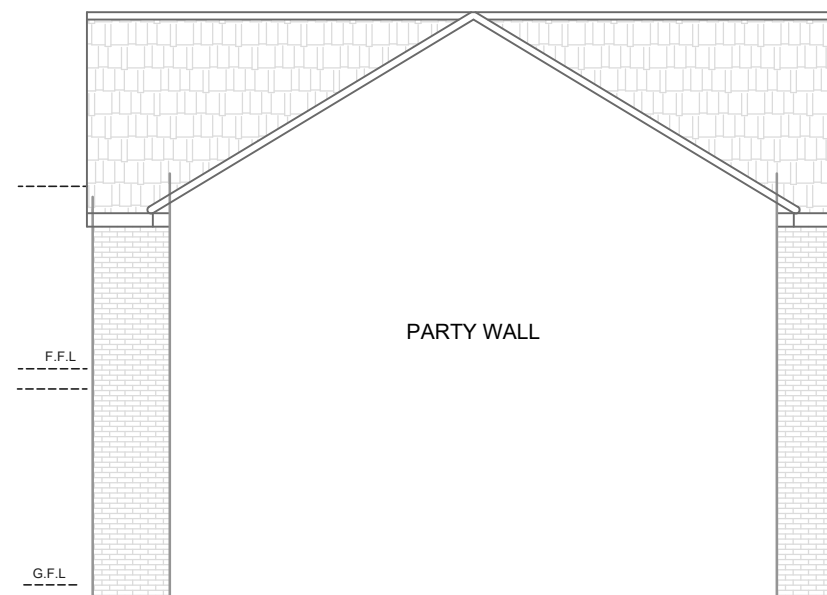
EXISTING REAR ELEVATION (REMAINS)
