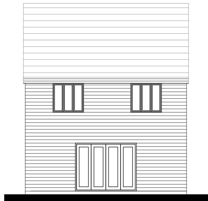
REAR ELEVATION
