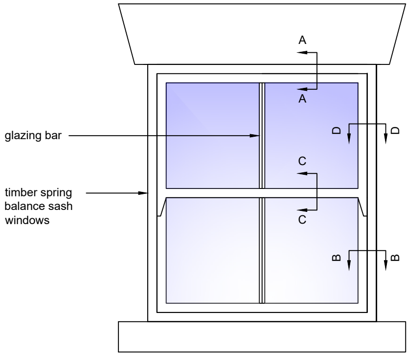
proposed window second floor scale 1-20
