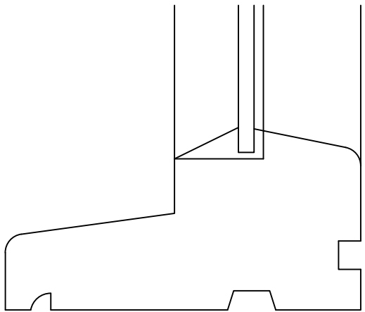
existing profile details scale 1-2
