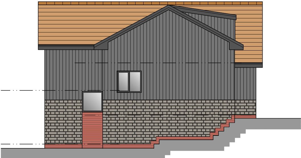
North West Facing Side Elevation
