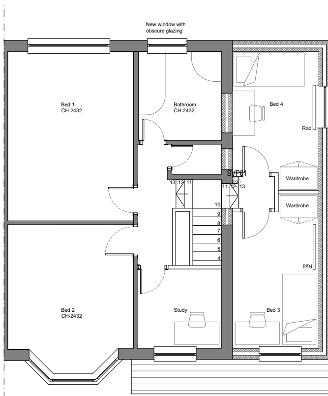
Proposed First Floor Plan Option 1 1:50
