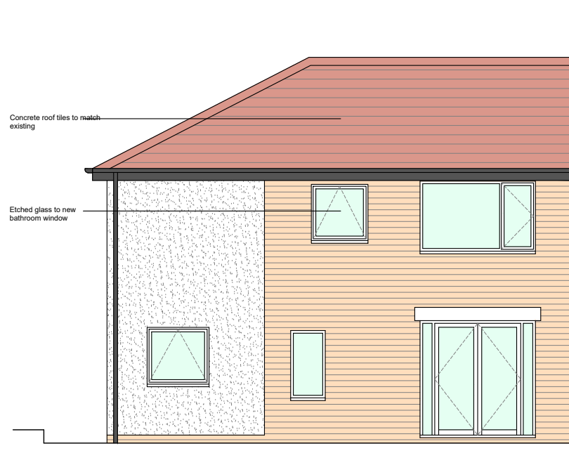
Proposed Rear Elevation Option 1 1:50
