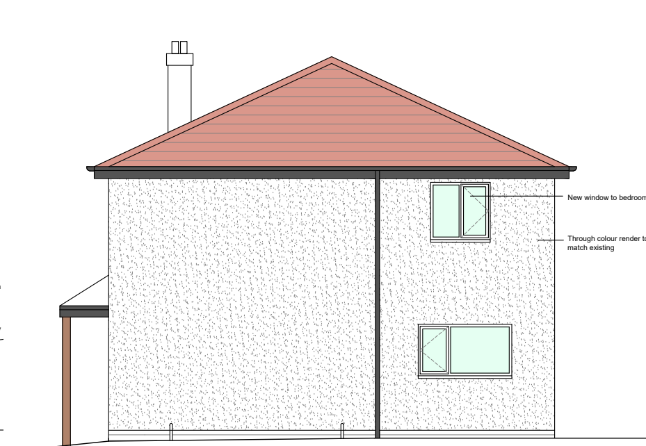
Proposed Side Elevation Option 1 1:50
