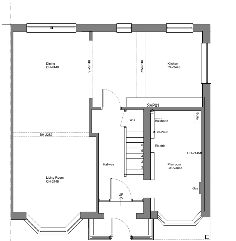
Proposed Ground Floor Plan Option 1 1:50
