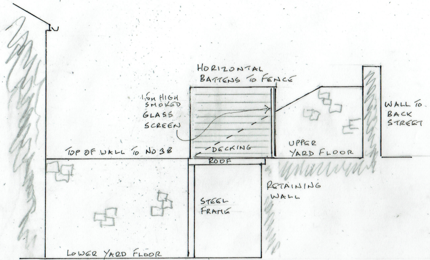
SECTION
