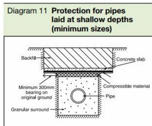
8 Shallow Drain Detail
