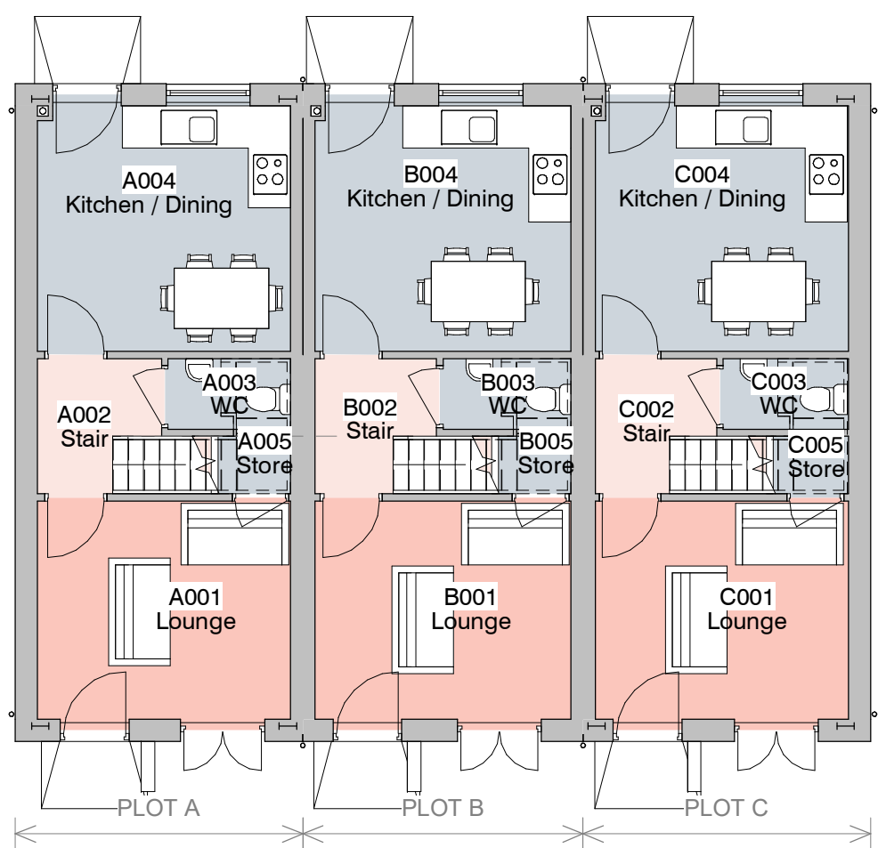
1. Level 0 - GA Proposed 1:100
