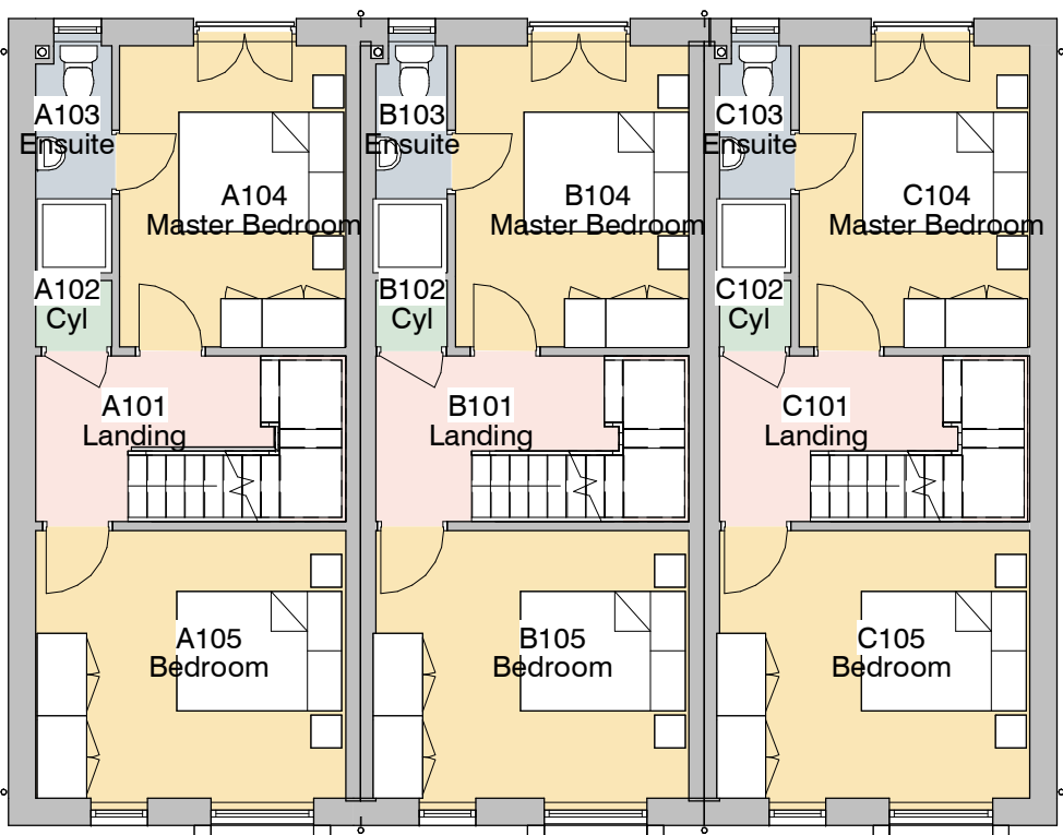
2. Level 1 - GA Proposed 1:100
