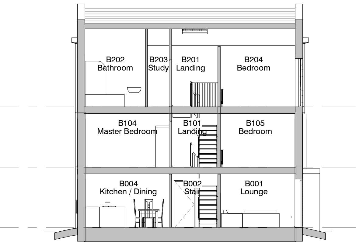
8. Section - Proposed - F-R 1:100
