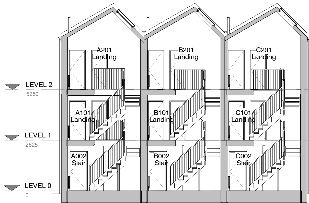
9. Section - Proposed - L-R 1:100
