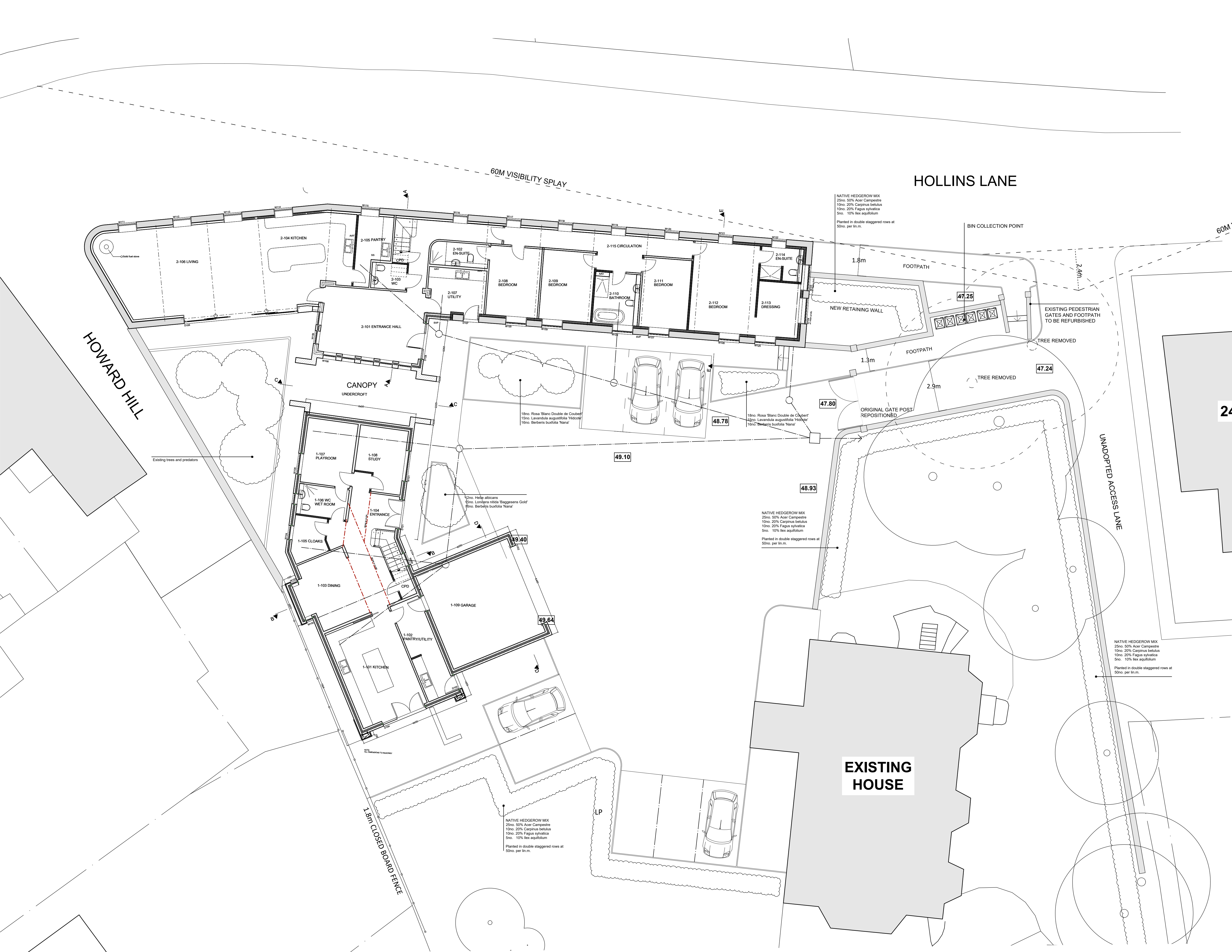
PROPOSED SITE with GROUND FLOOR LAYOUT
