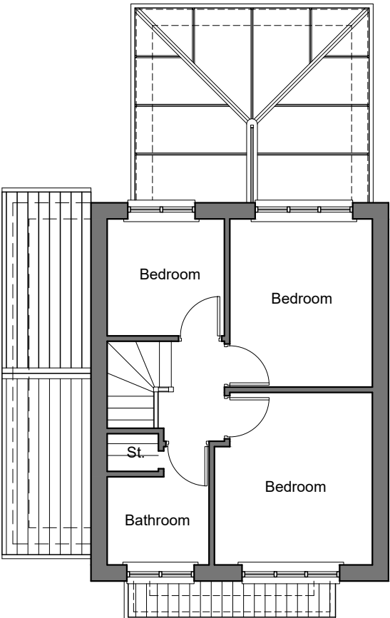
Existing 1/F Plan
