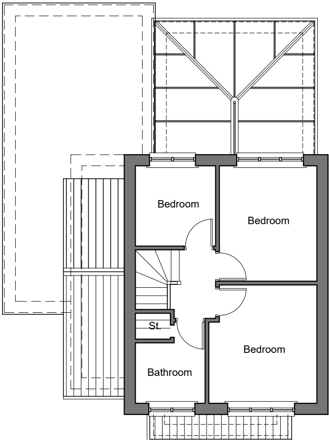
Proposed 1/F Plan
