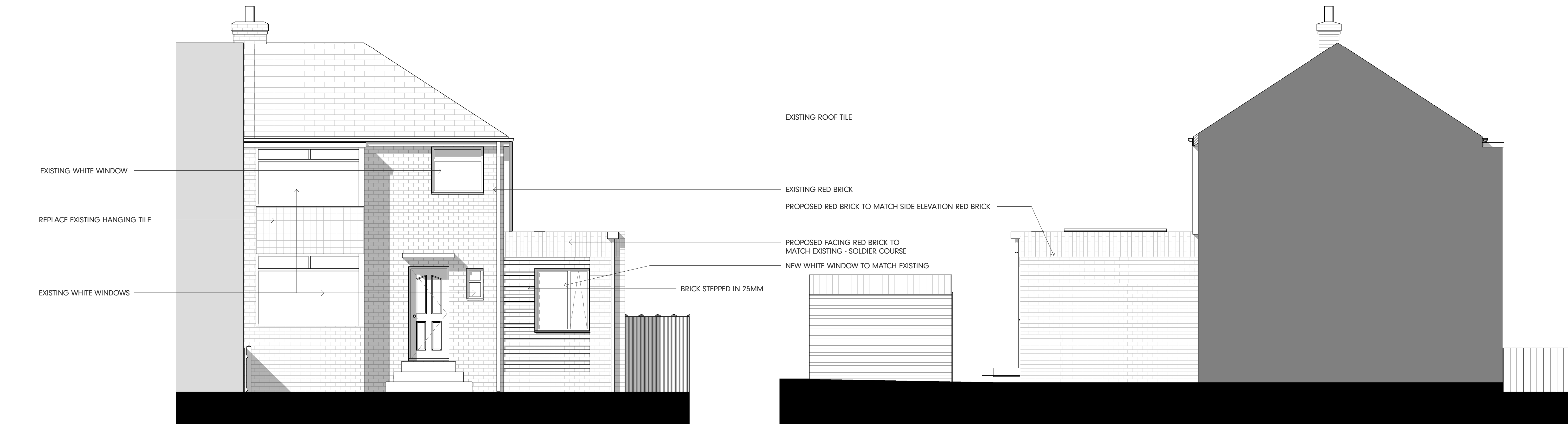
Proposed South Facing Elevation
