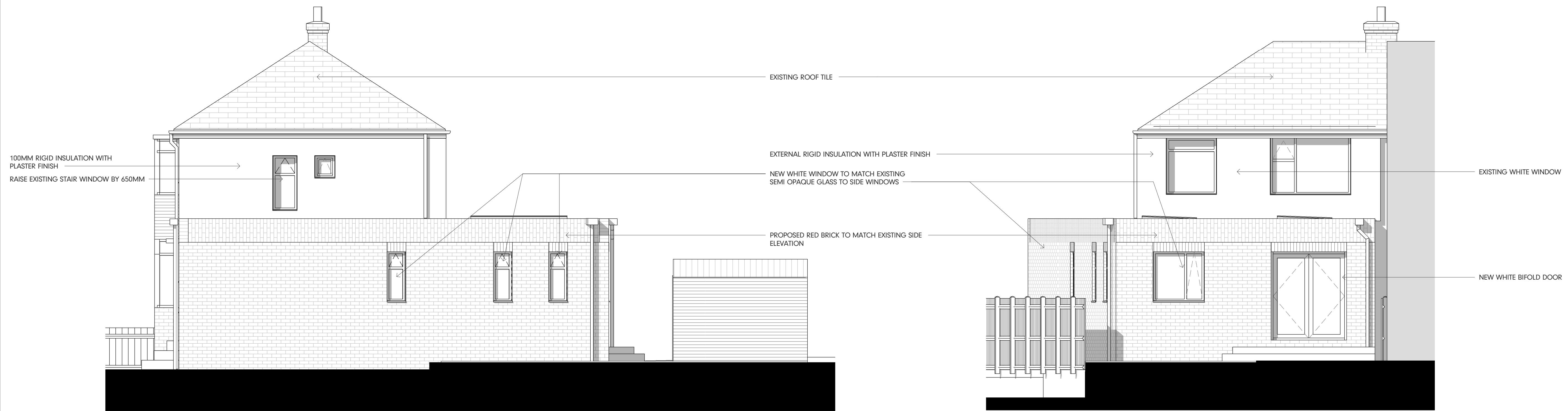
Proposed East Facing Elevation
