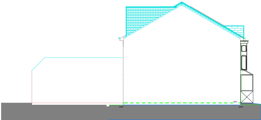
PROPOSED SIDE A ELEVATION
