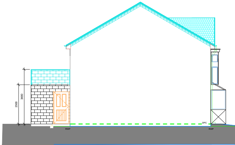
EXISTING SIDE A ELEVATION
