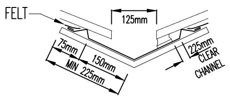
PITCHED VALLEYS KEY DIMITIONS
