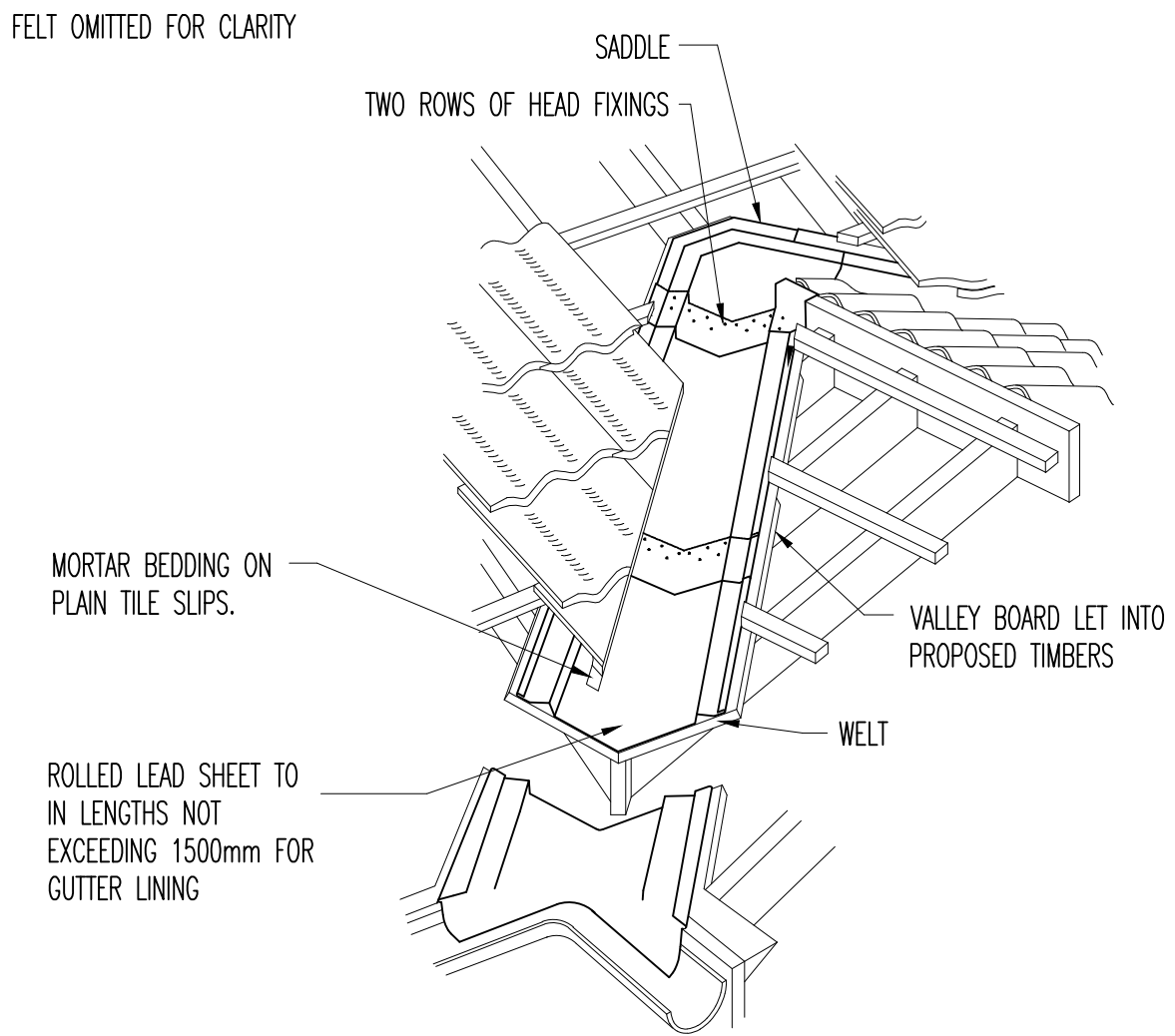
PITCHED VALLEYS KEY DIMITIONS
