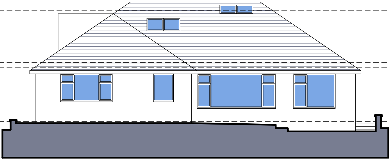
FRONT ELEVATION (East)
