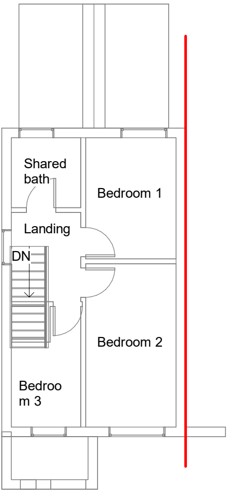
4 First Floor - Proposed 1 : 100
