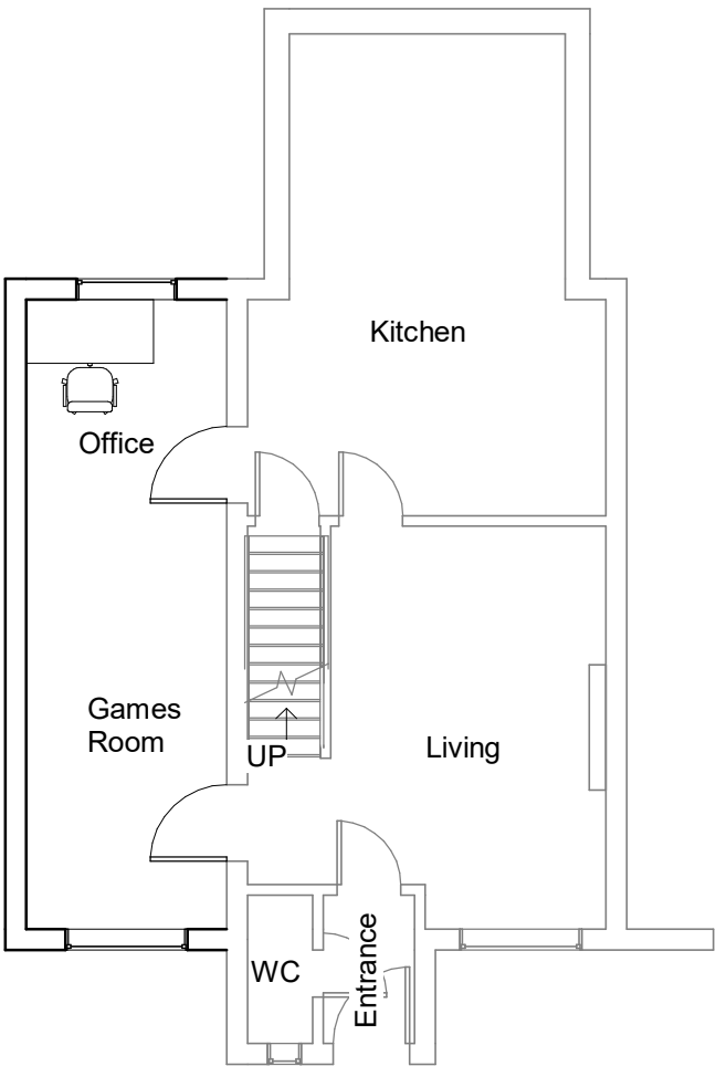
3 Ground Floor - Proposed 1 : 100
