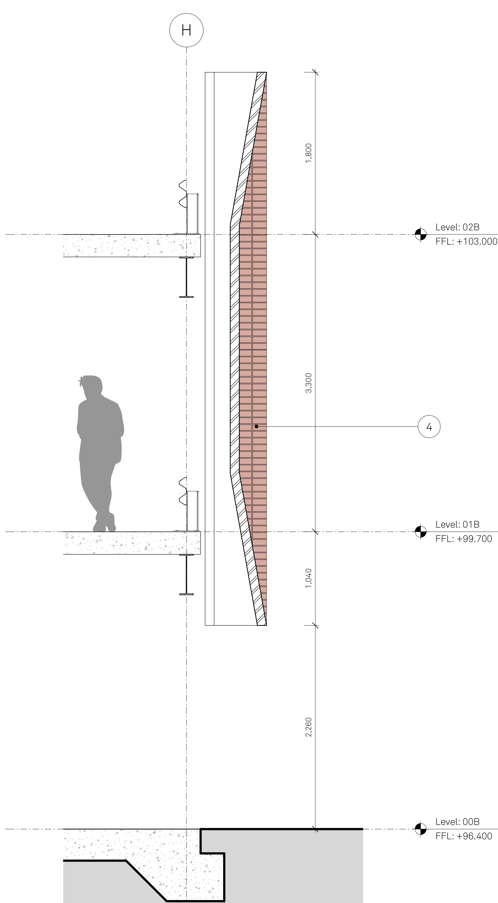
A Study Bay 2 - Section Detail THROUGH BRICK 'FINS'
