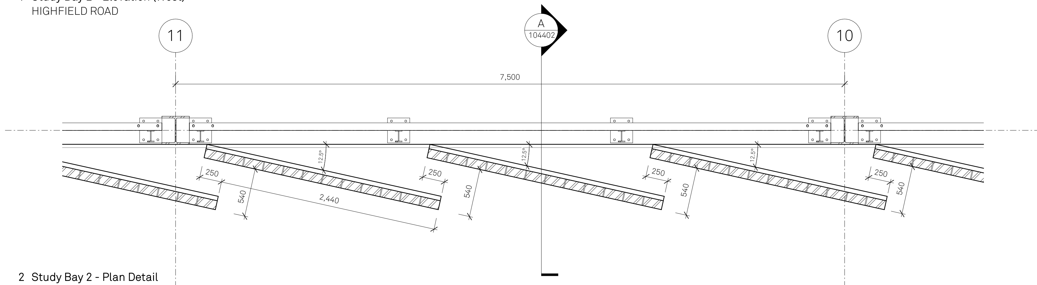
2 Study Bay 2 - Plan Detail TYPICAL FLOOR
