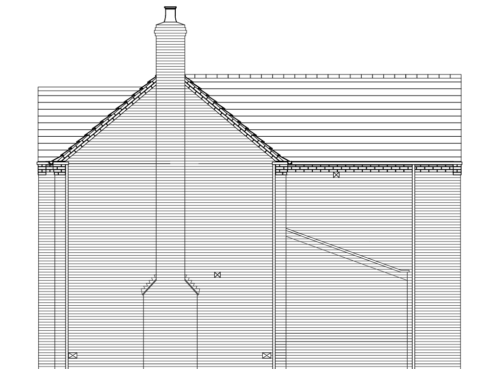
SIDE / REAR ELEVATION
