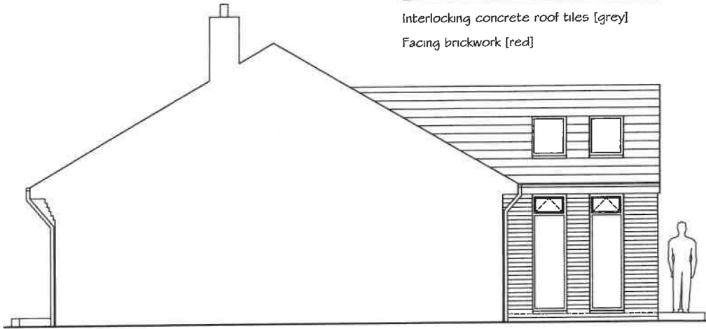
PROPOSED SOUTH EAST SECTIONAL ELEVATION 1:100 @ A4 [AS VIEWED FROM NO 4]
