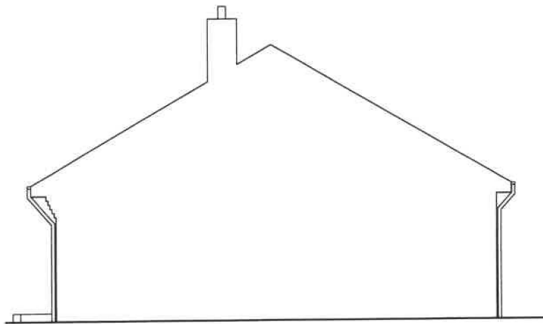
EXISTING SOUTH EAST SECTIONAL ELEVATION 1:100 @ A4 [AS VIEWED FROM NO 4]
