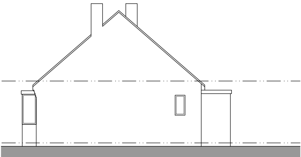
South Facing Side Elevation
