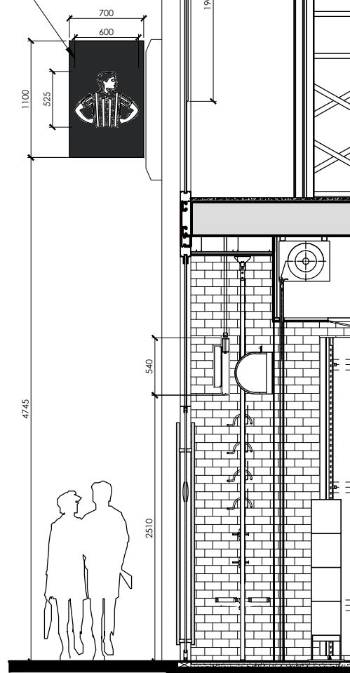
Proposed shopfront section A-A 1:50 @ A3
