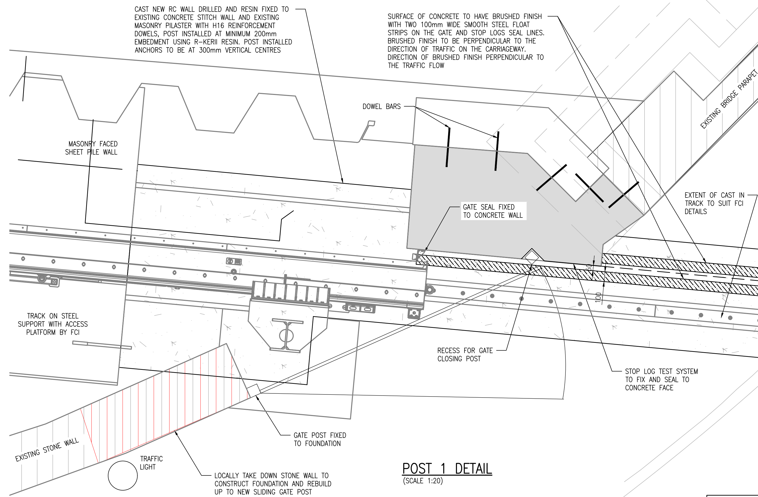
ROAD LEVEL PLAN (SCALE 1:50)
