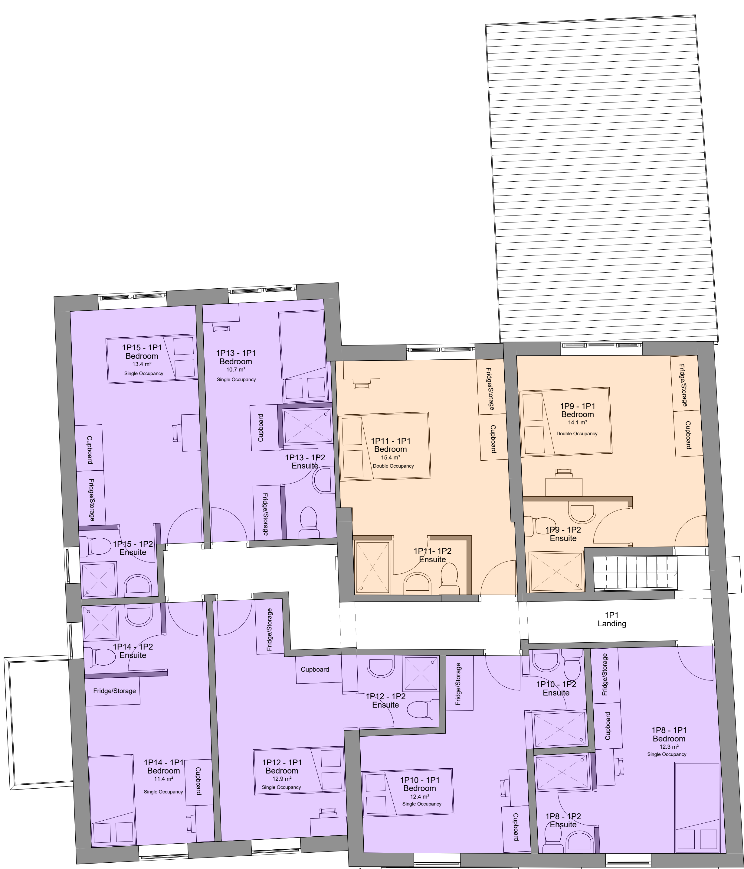
2 Level 1 - Proposed 1 : 50
