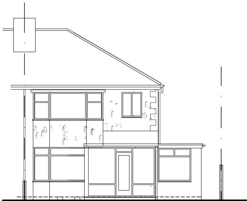
FRONT EXISTING
