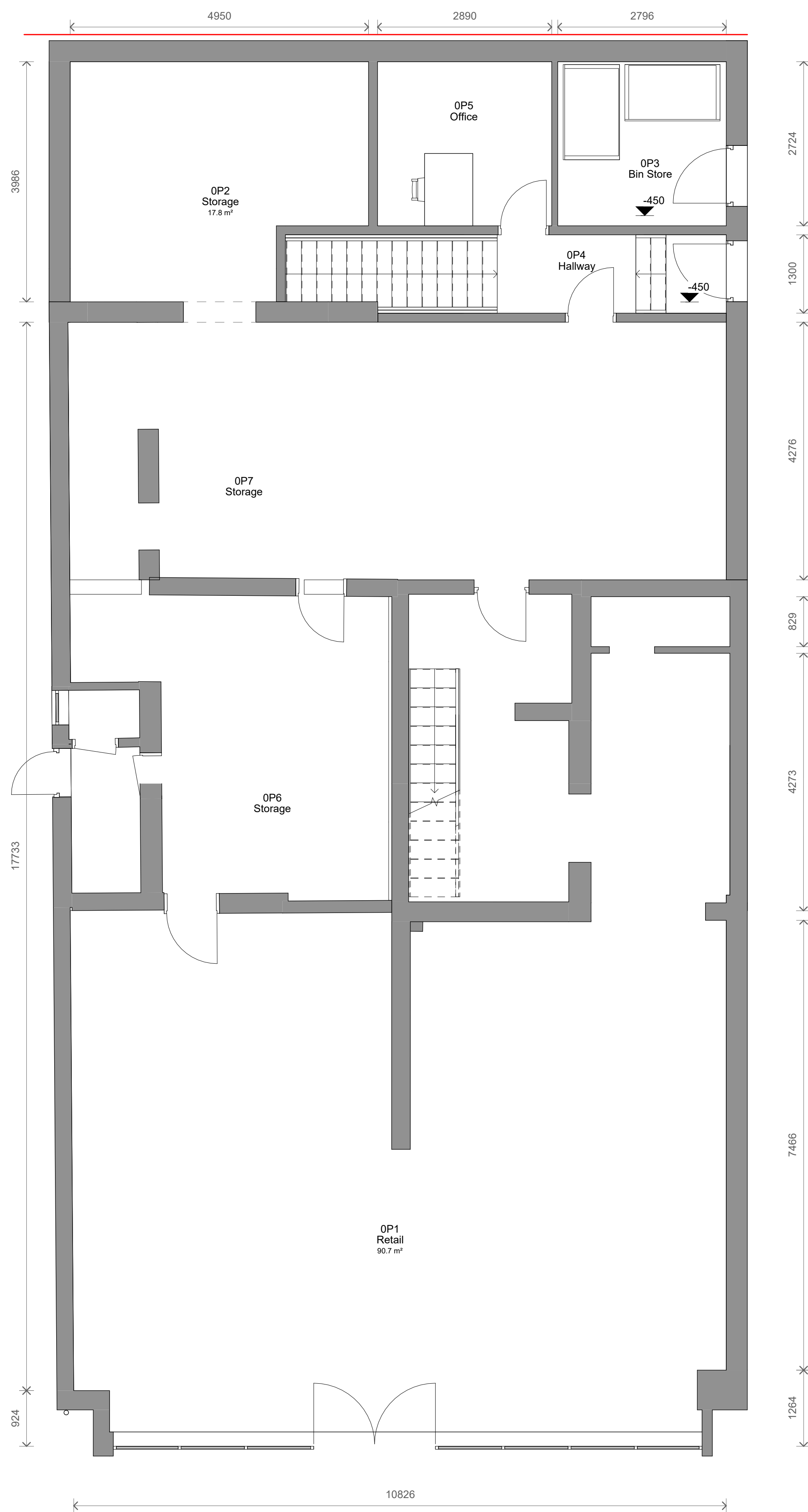
2 Level 0 - Proposed 1 : 50
