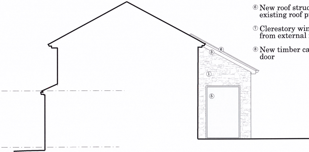
Elevation D
