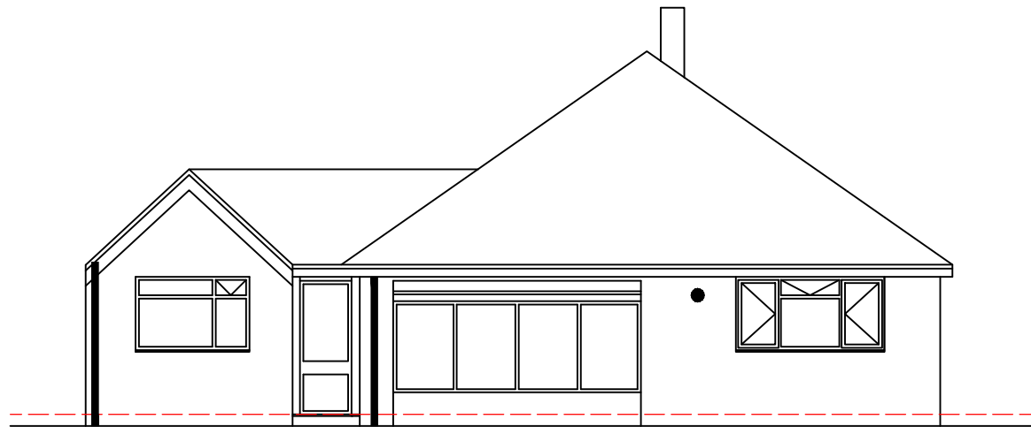
REAR ELEVATION 1:100
