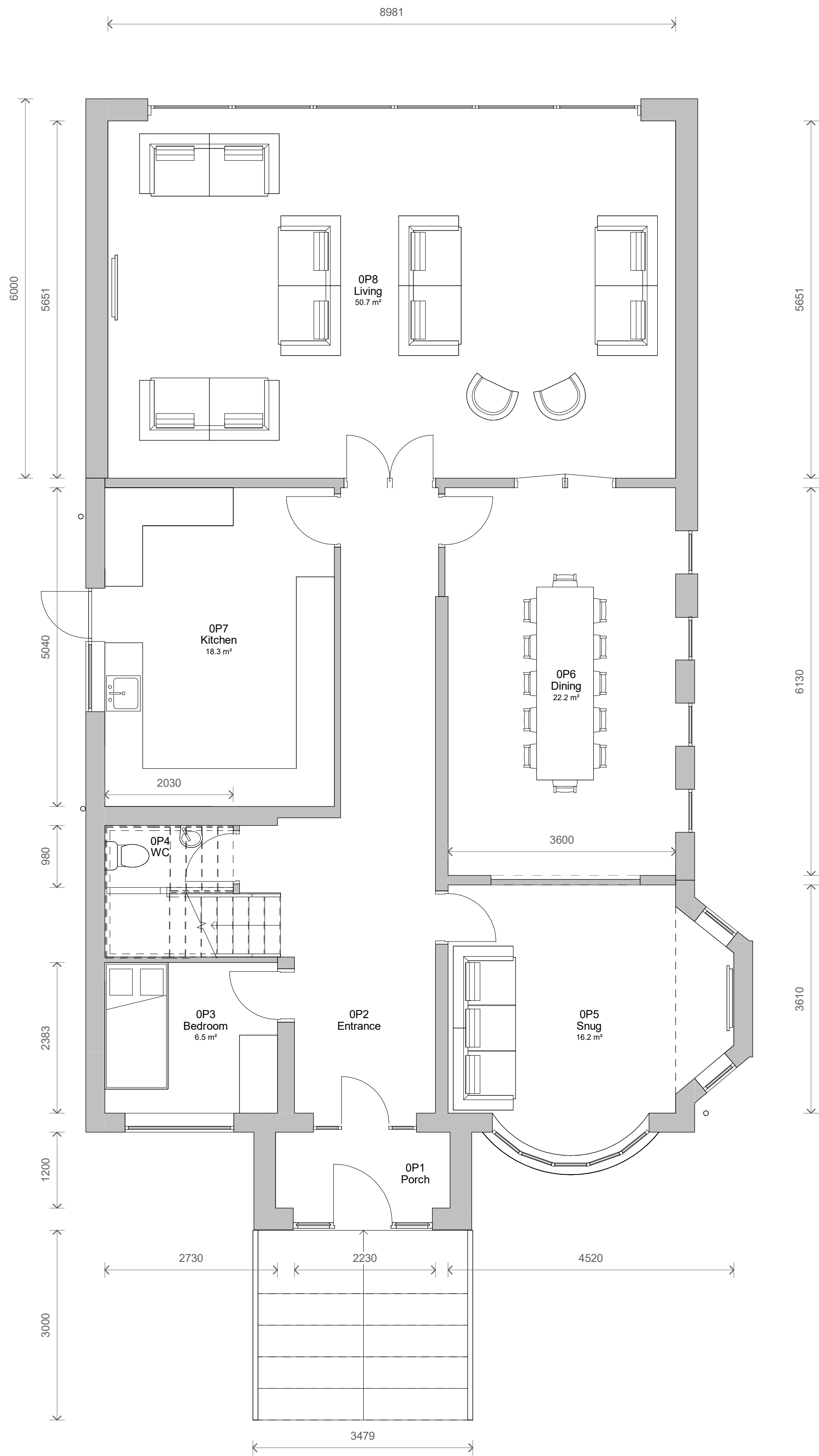
1 Level 0 - Proposed 1 : 50
