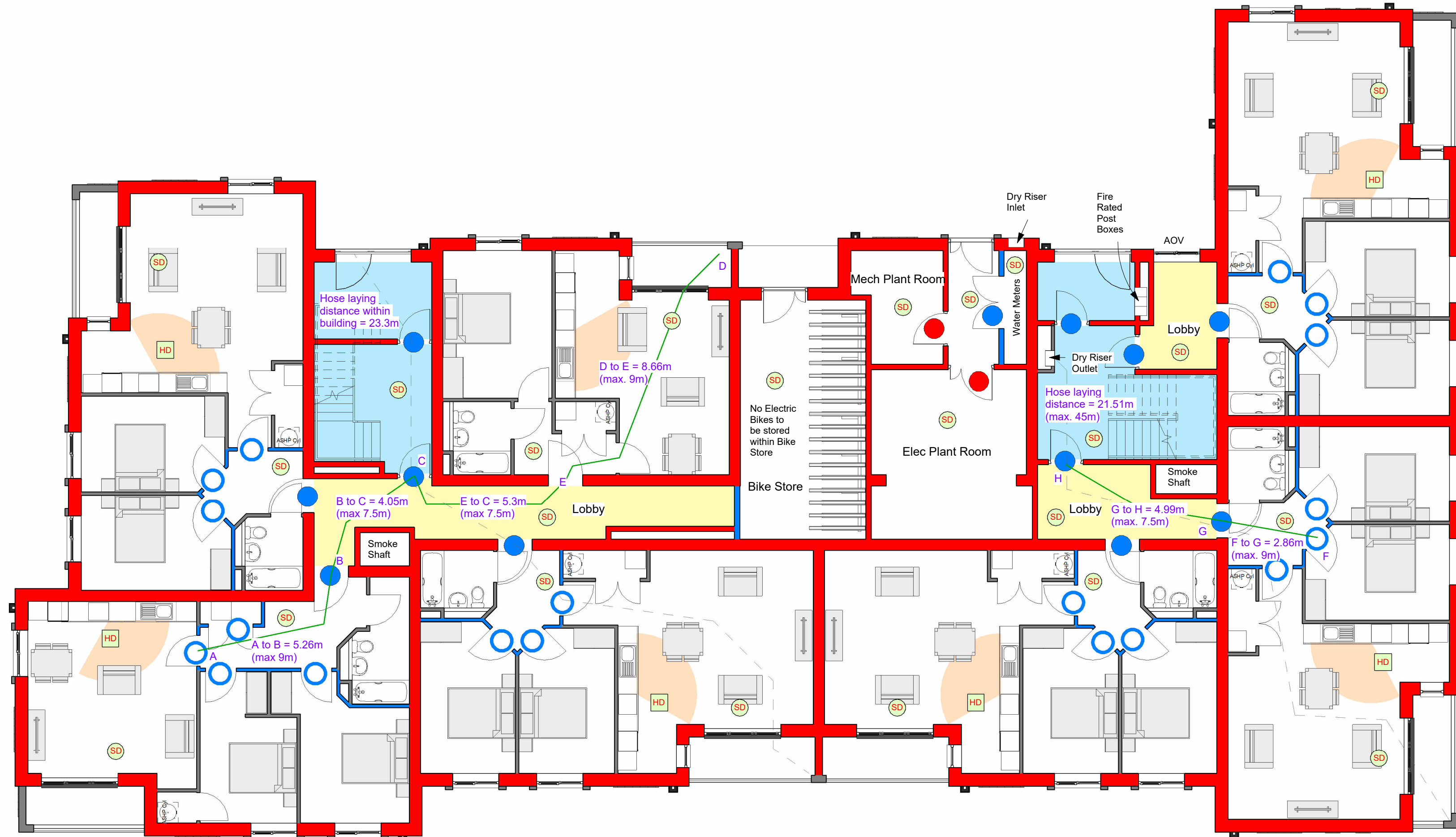
2 Block A_L1 First Floor Fire Plan 1 : 100
