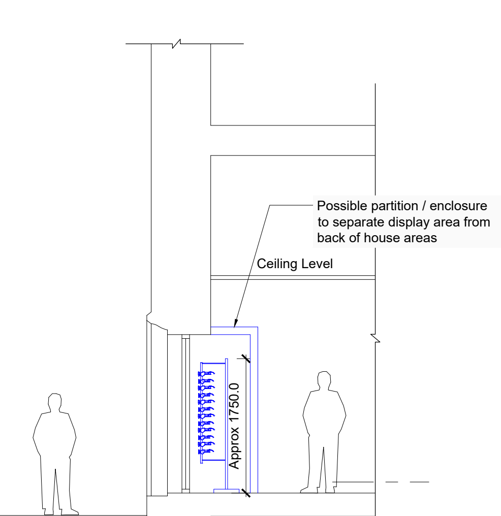
Section Detail 4 Scale 1:50
