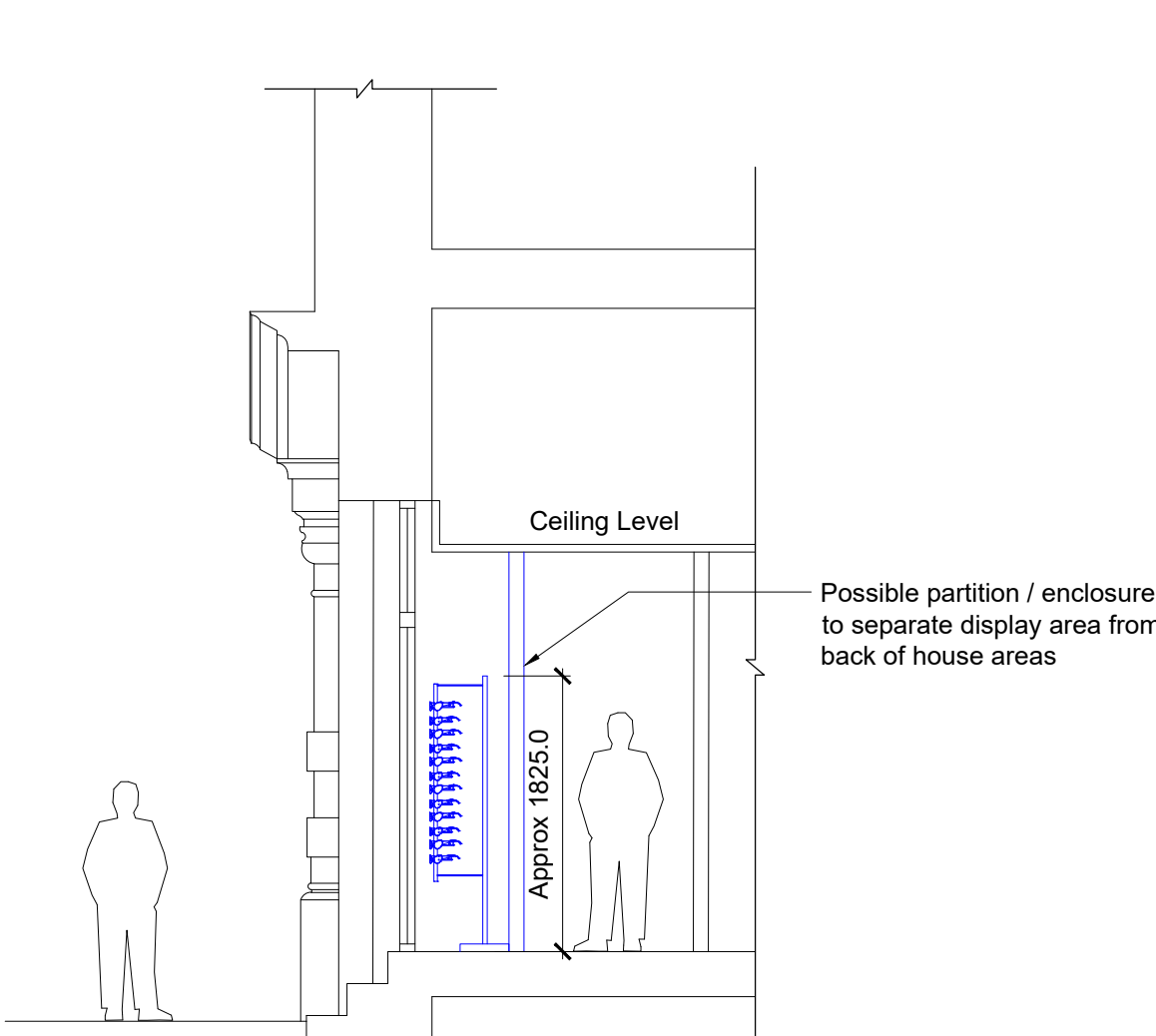
Section Detail 5 Scale 1:50
