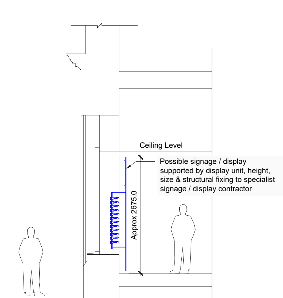
Section Detail 6 Scale 1:50
