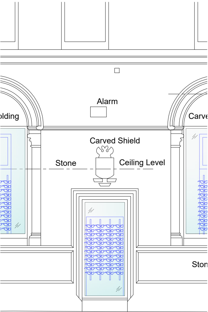
Elevation Detail 4 Scale 1:50
