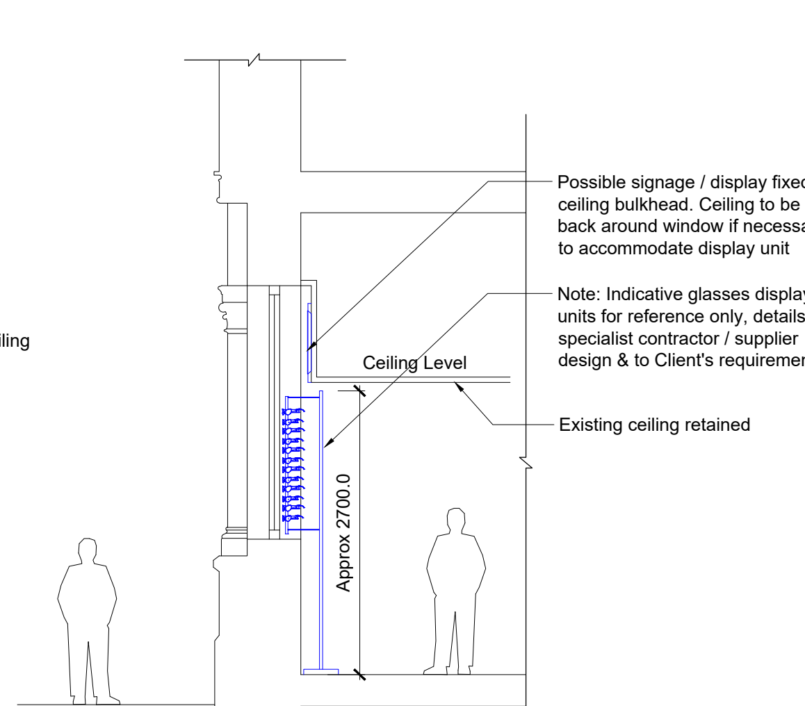
Section Detail 3 Scale 1:50
