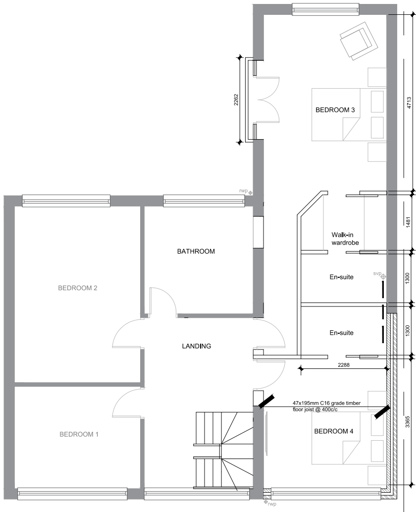
First floor
