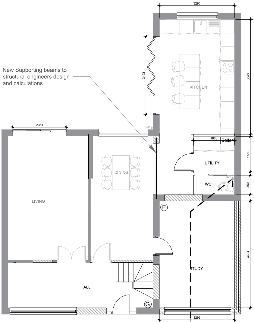
Ground floor
