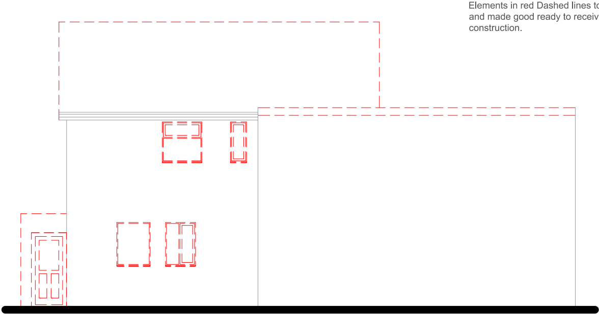
Side Elevation
