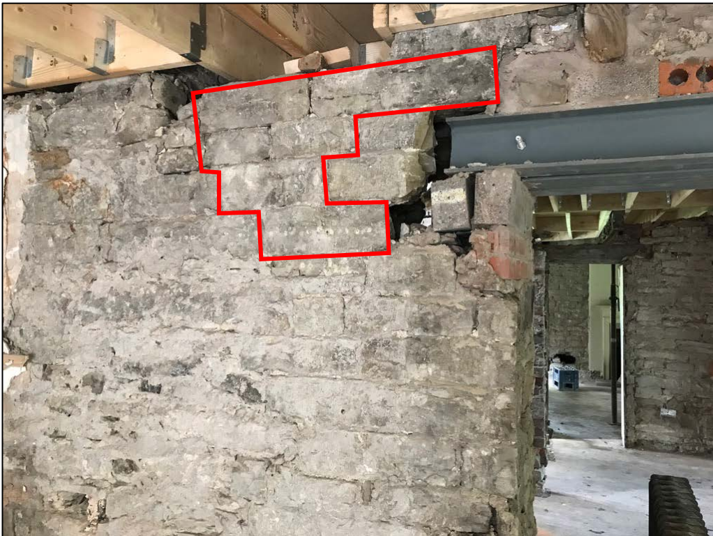
5.7 Proposed exposed stone section (2) to remain visible within former external wall of c. 1739.
