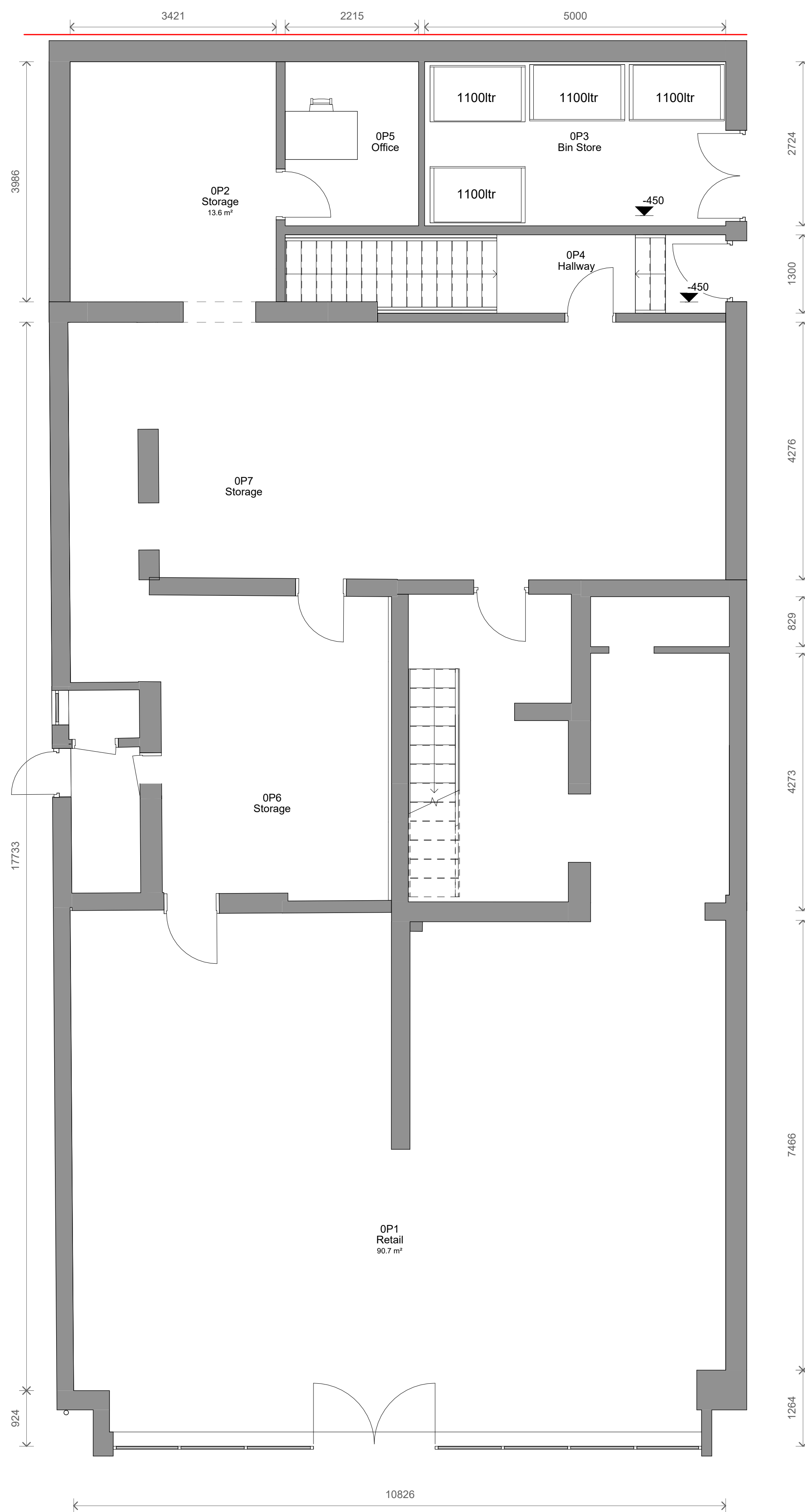
2 Level 0 - Proposed 1 : 50
