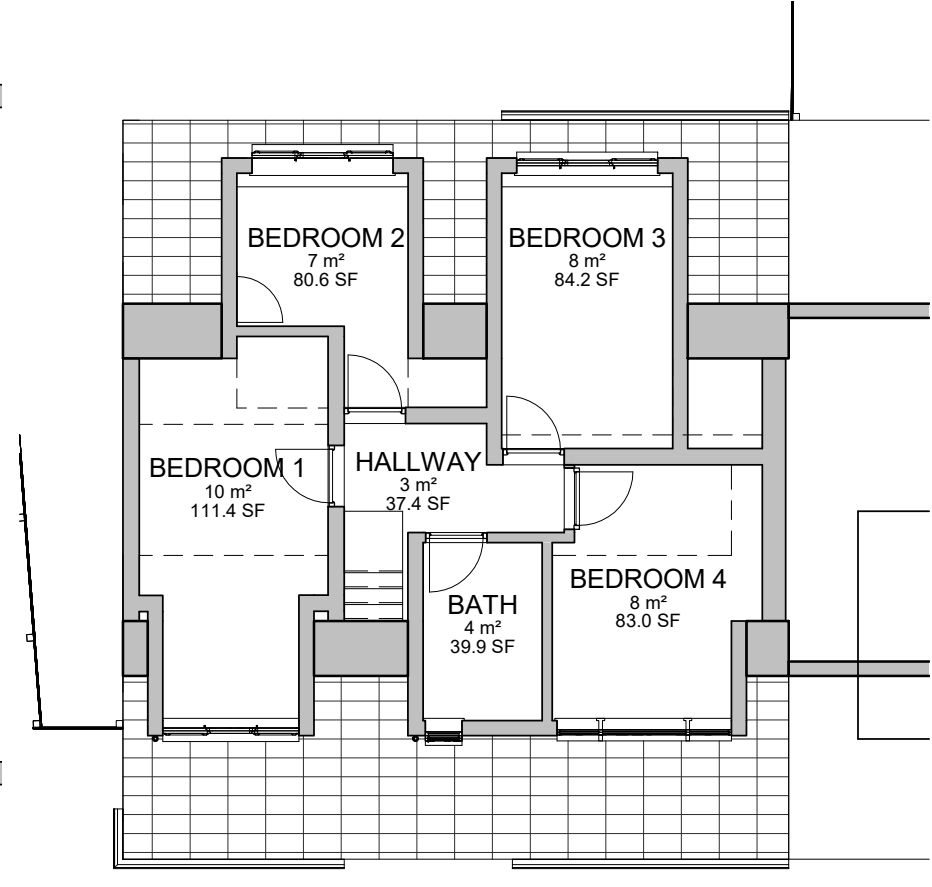
2 Existing First Floor Plan 1 : 100
