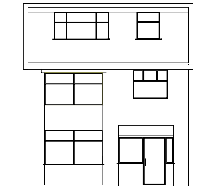
Rear Elevation
