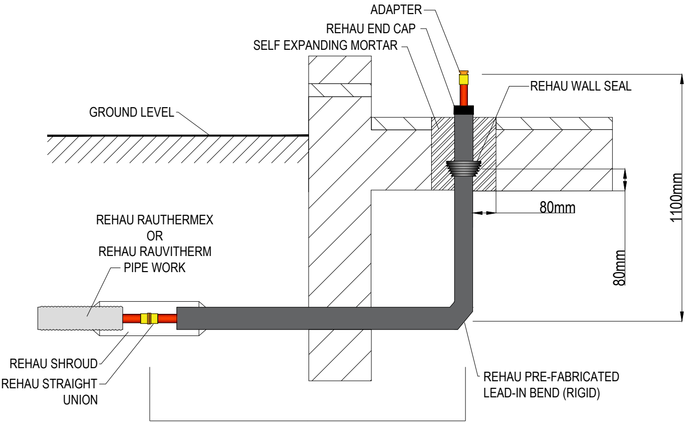
REHAU PRE-FABRICATED LEAD-IN BEND INSTALLATION DETAIL SCALE: NTS
