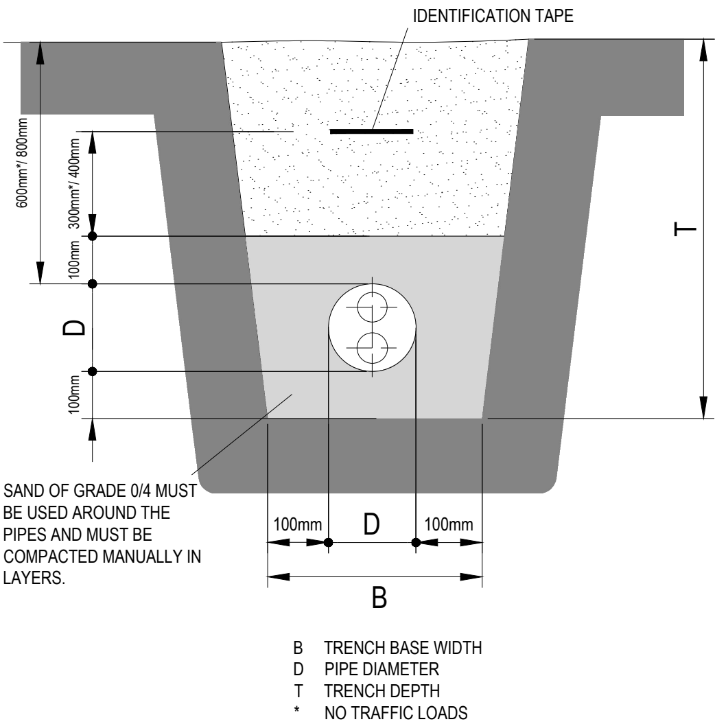
REHAU DUO PREINSULATED PIPEWORK TRENCH DETAIL SCALE: NTS
