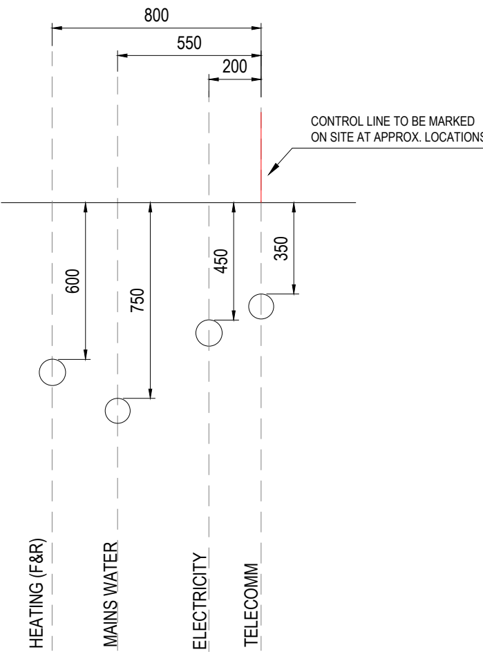
COMBINED SERVICES TRENCH DETAIL SCALE 1:20
