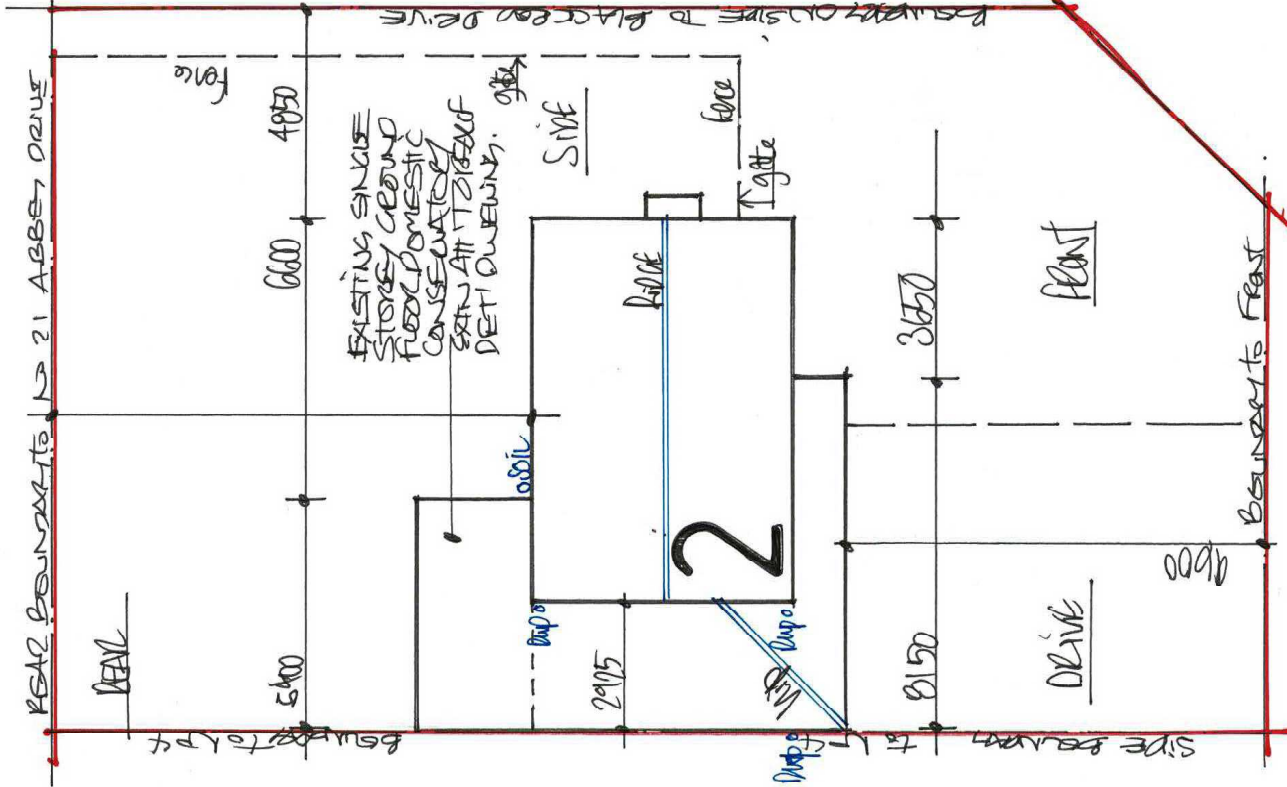
1:125 EXISTING "BLOCK PLAN".
