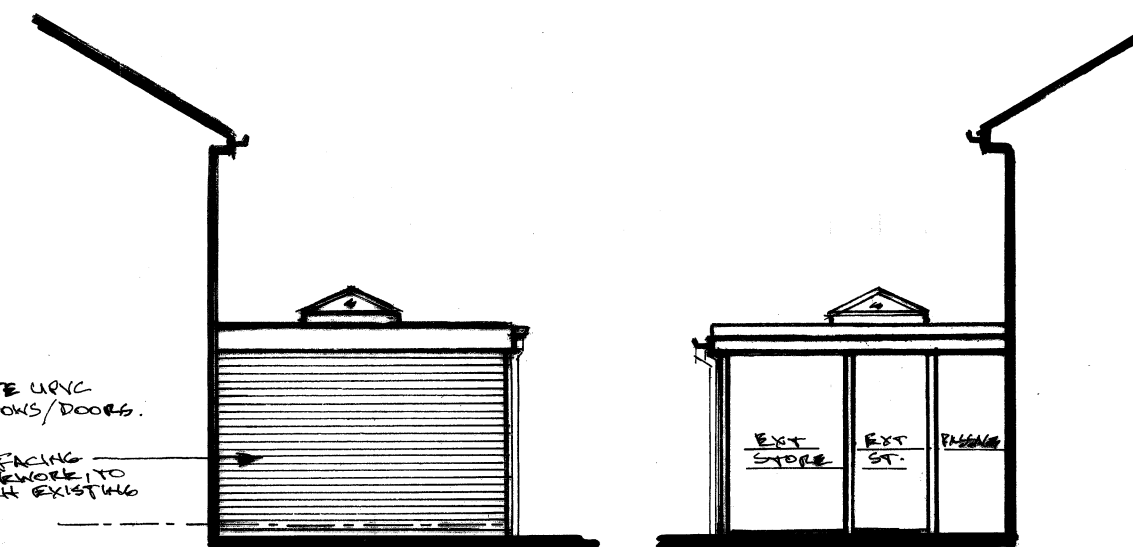
PROPOSED L.H. SIDE ELEV. (FROM REAR)
